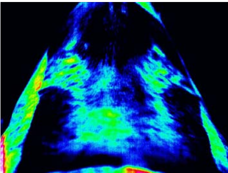
Left: Thermal image of a horse’s back during a saddle-fitting seminar. The saddle put increased pressure over the left side of the horse’s back, and impinged on the left thoracic spine. Thermography is a useful saddle-fitting tool, but should be combined with a certified saddle-fitter for best results.
