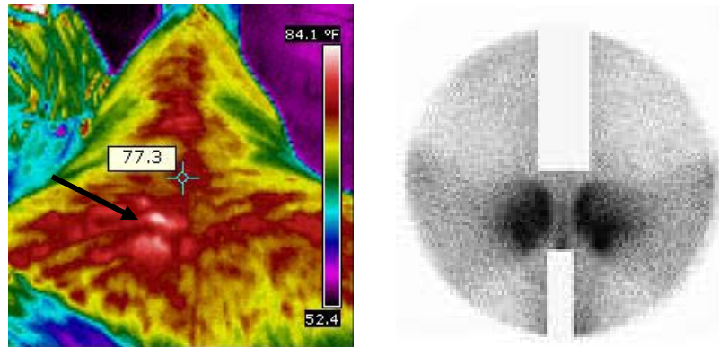
Above: Image at left is a thermal scan showing increased heat over the sacroiliac/tuber sacrale region of a horse (arrow). At right is a nuclear scintigraphy image of the same region on a different patient (from Langfordvets.co.uk)
